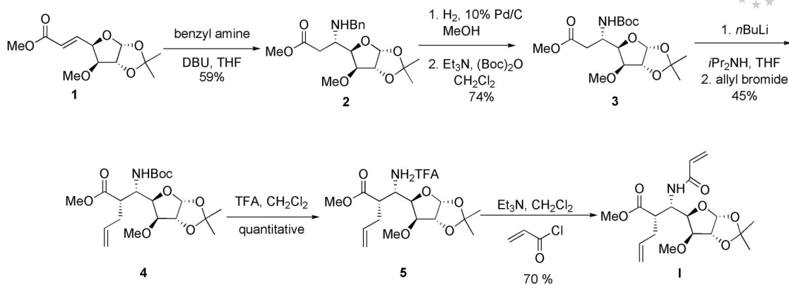
Scheme 1. Synthesis of \beta -Caa I .
