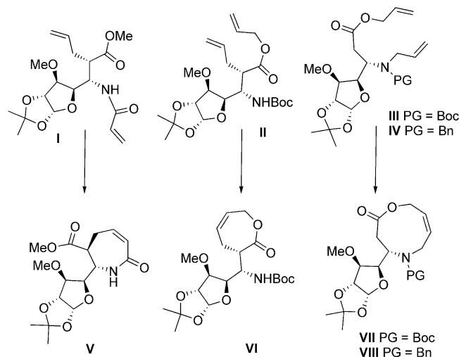
Figure 1. Cyclization of amino acid dienes I , II , III , IV .
