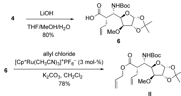
Scheme 2. Preparation of II .
