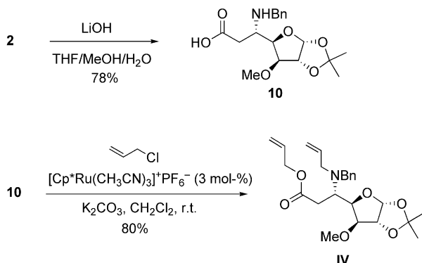
Scheme 4. Synthesis of IV .
