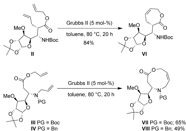
Scheme 5. Synthesis of cyclized \beta -amino acid derivatives.
