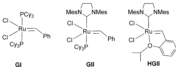
Figure 2. Metathesis catalysts used for RCM reactions.
