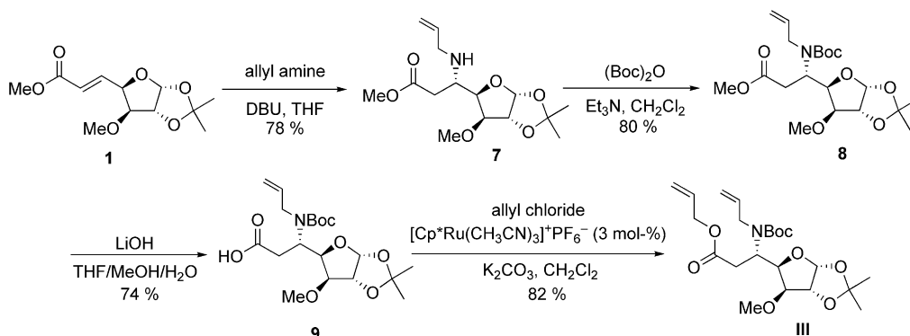
Scheme 3. Synthesis of \beta -Caa III .
